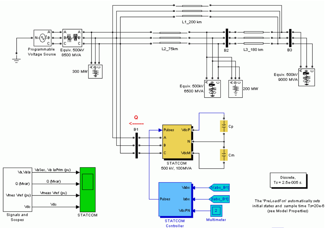
Figure 5-6: SPS Model of the 100 Mvar STATCOM on a 500 kV Power System (power_statcom_gto48p)
