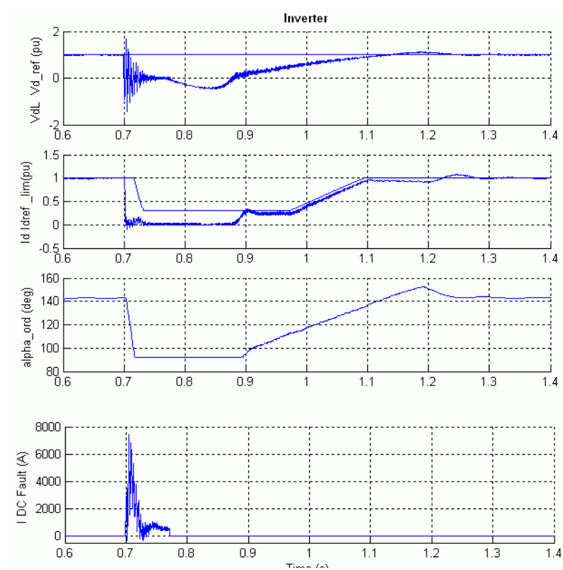
Figure 5-13: DC Line Fault on the Rectifier Side
