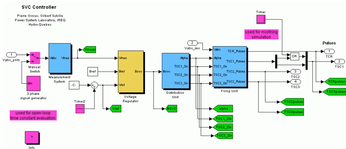
Figure 5-5: SVC Control System
