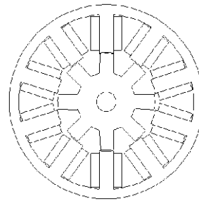
Four-phase 8/6 SRM
