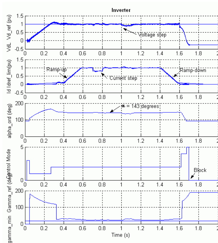
Figure 5-10: Startup/Stop of the DC System and Step Applied on the Current and Voltage Reference
