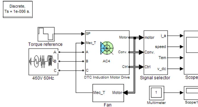
Figure 4-5: Induction Motor Drive Example Circuit
