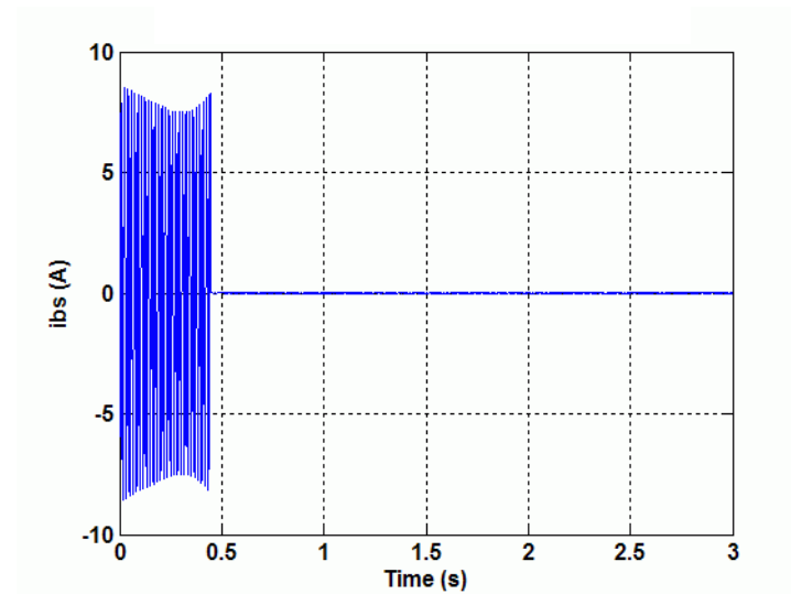
Auxiliary Winding Current in Capacitor-Start Operation Mode
