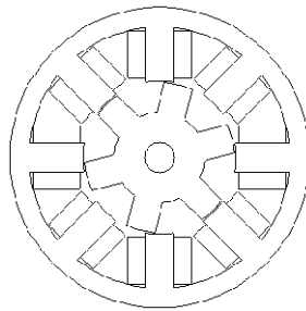
Three-phase 6/4 SRM
