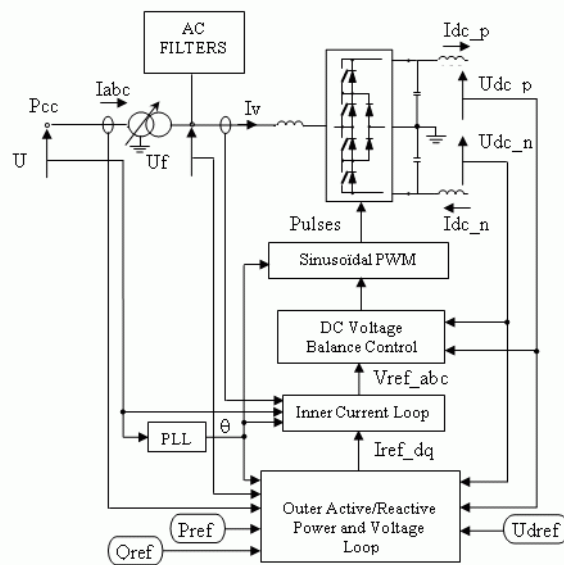
Figure 5-18: Overview of the Control System of a VSC Converter and Interface to the Main Circuit
